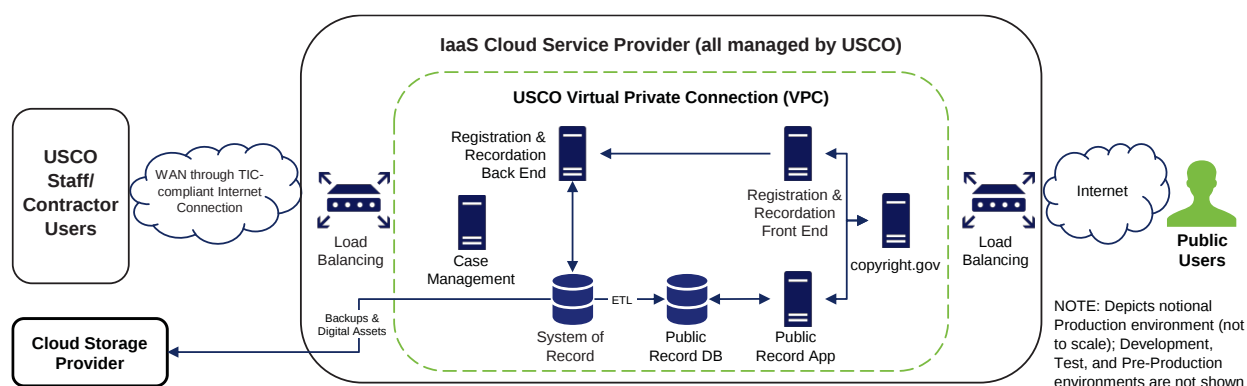
Figure 3.3.1-3: Notional IaaS-focused Architecture
